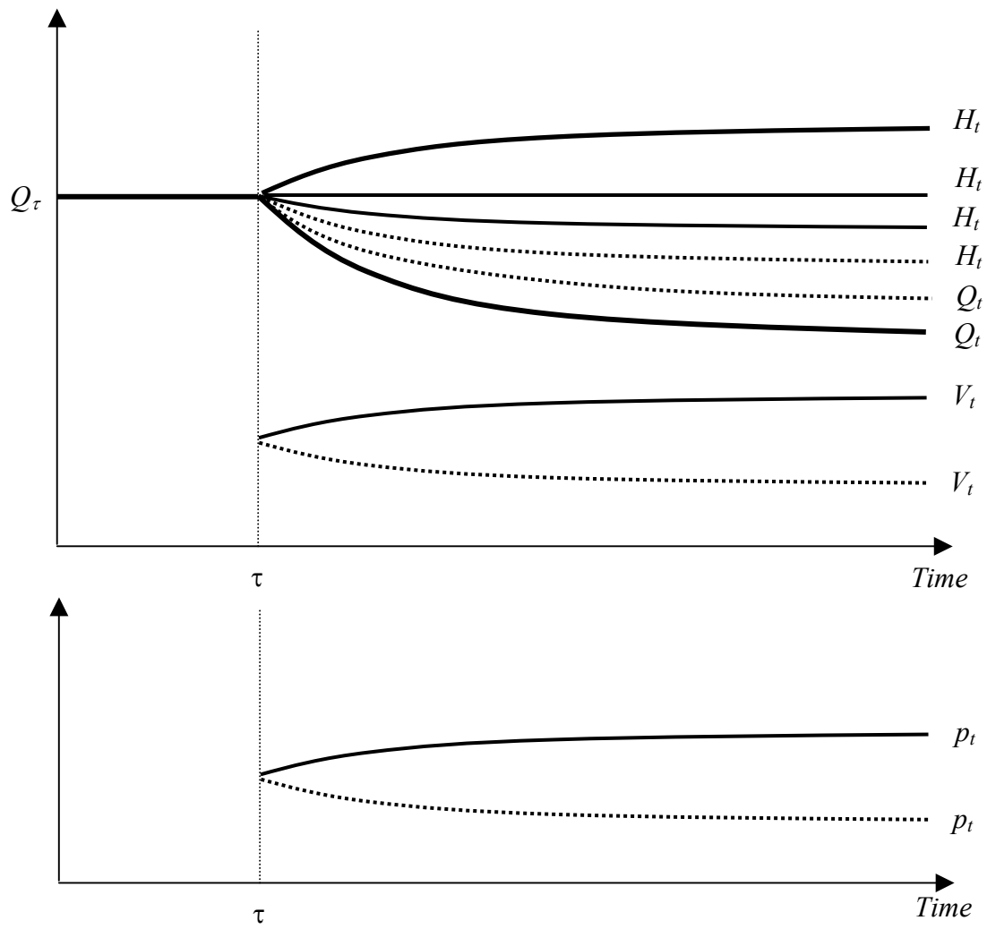
Figure 3: Time paths of quota price, harvest, and violations
