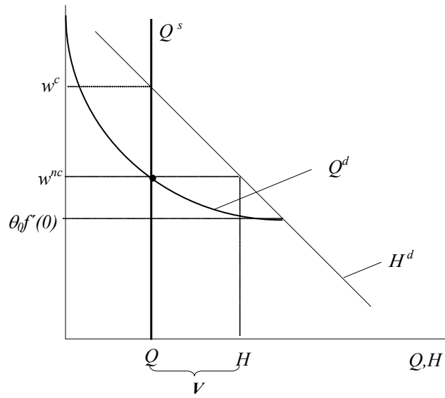
Figure 2. Equilibrium quota market under non-compliance
