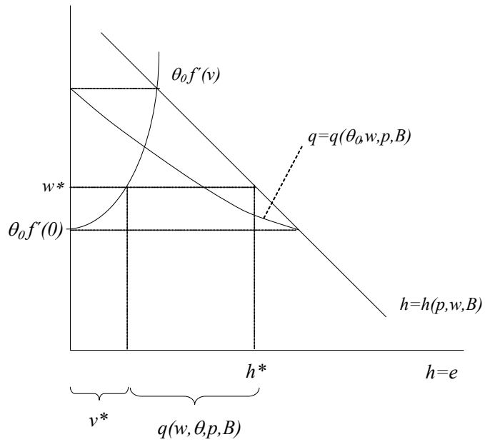
Figure 1. Fisherman behavior under imperfectly enforced ITQ system
