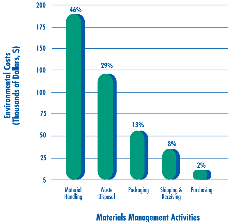
Figure 4: Pareto Diagram
