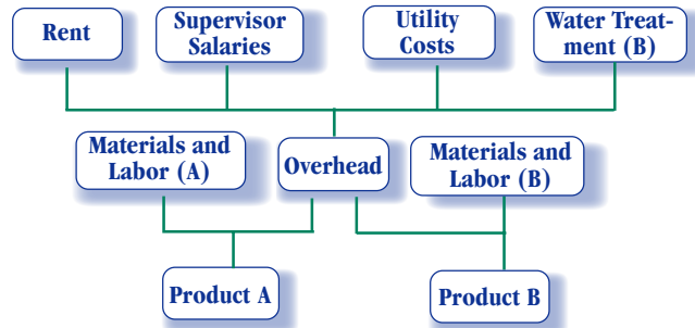
Figure 2: Improved Allocation
