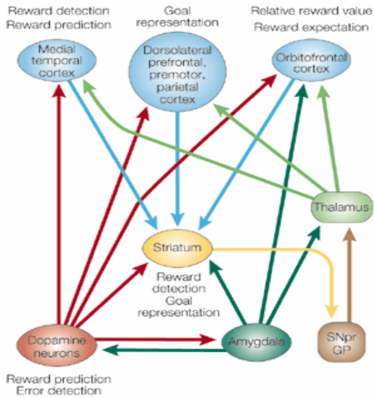
Figure 4: Hypothesized neural circuitry of reward processing (Schultz, 2000)
